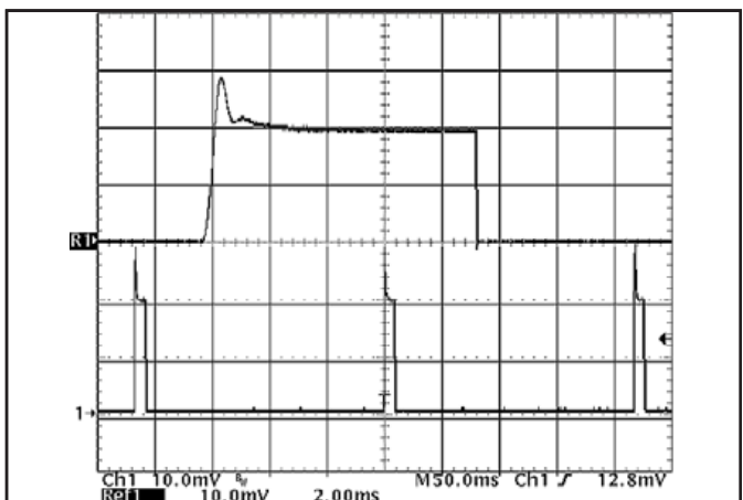
Figure 18: Load current ( 20\ \text{A}/\text{div} ) as a function of time when the converter turns on into a 1\ \text{m}\Omega short circuit. Top trace ( 2\ \text{ms}/\text{div} ) is an expansion of the on-time portion of the bottom trace.
